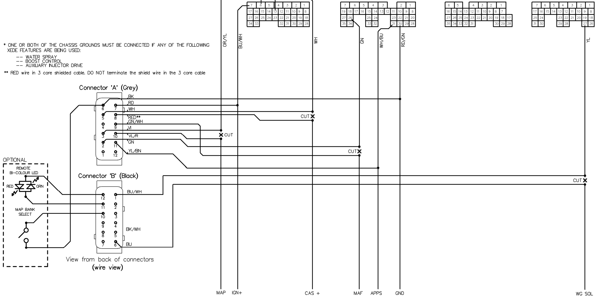
ECU Connector View from back of connectors (wire view)
